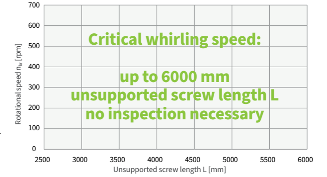
Critical whirling speed ZA-100
