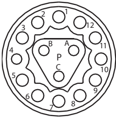
Intercontec Itec 915 15-pole, female - cable side
