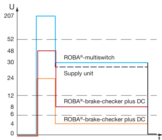
Time Diagram: Operation of the brake
