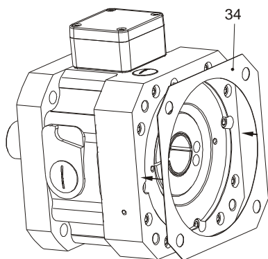
Fig. 7: Input-side seal
