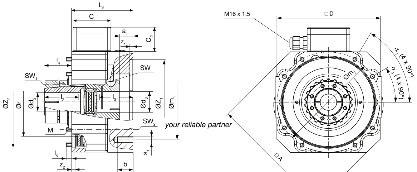
Fig. 6 Type 899.111. Brake module without output flange with plug-in shaft coupling (Clamping hub motor-side)
