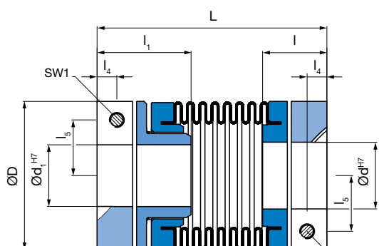
Type 933.533.1 without keyway Type 933.566.1 with keyway
