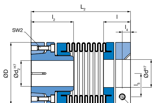
Type 933.535.1 without keyway Type 933.567.1 with keyway
